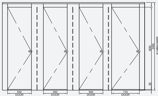
Elevation View
